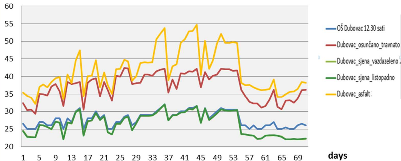
Current air temperature at 12.30 h and surface temperatures of different surfaces in warm and hot days from April 22 th - September 21 st 2018. on the atmospheric station GLOBE Elementary school Dubovac, Karlovac
