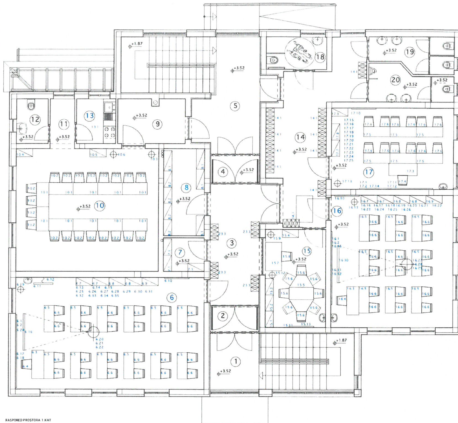
RASPORED PROSTORA 1.KAT
