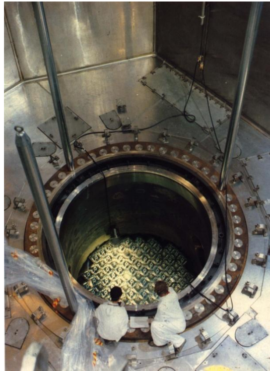
NEK - Westinghouseov nuklearni reaktor
